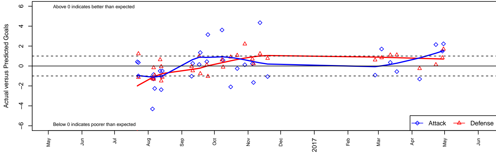
WUSC White B04 Dots are actual minus expected GF (blue circles) and GA (red triangles). Blue line is smoothed change in attack strength. Red is smoothed change in defense strength.
